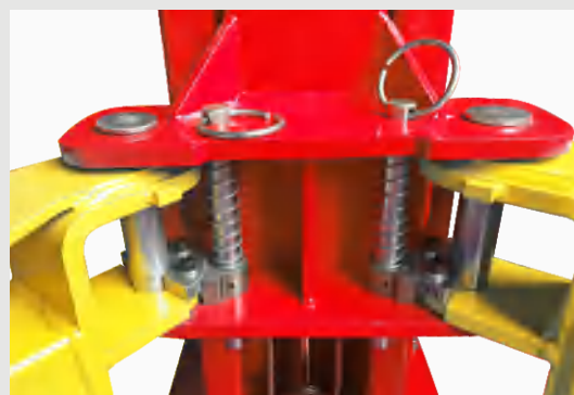
• Lifting arms lock automatic release device, high strength gear rack, more stable and reliable.
